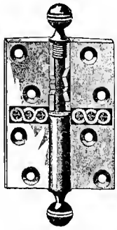
Fig. 2586. ACORN BUTT-HINGE. LOOSE-PIN REVERSIBLE Knuckle broken open to show washer-bearing.
